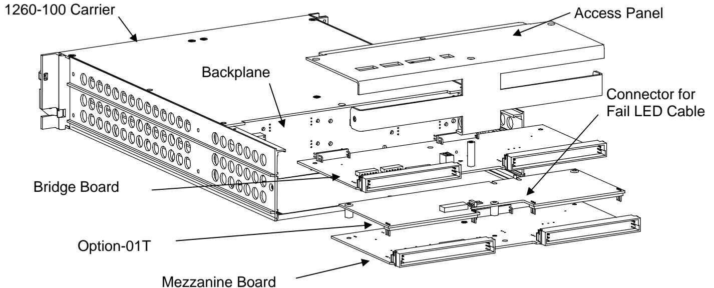
Figure 2-1, Installing the Option-01T in the 1260-100 (For the 1260-101 single-slot carrier, see text below)
